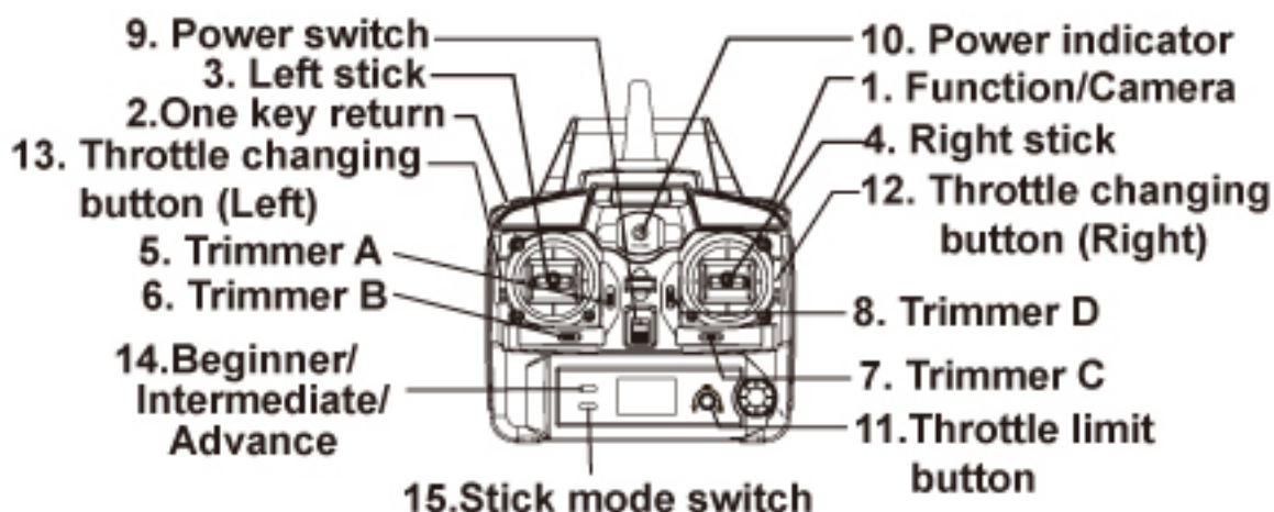
Remote Controller(Transmitter)
